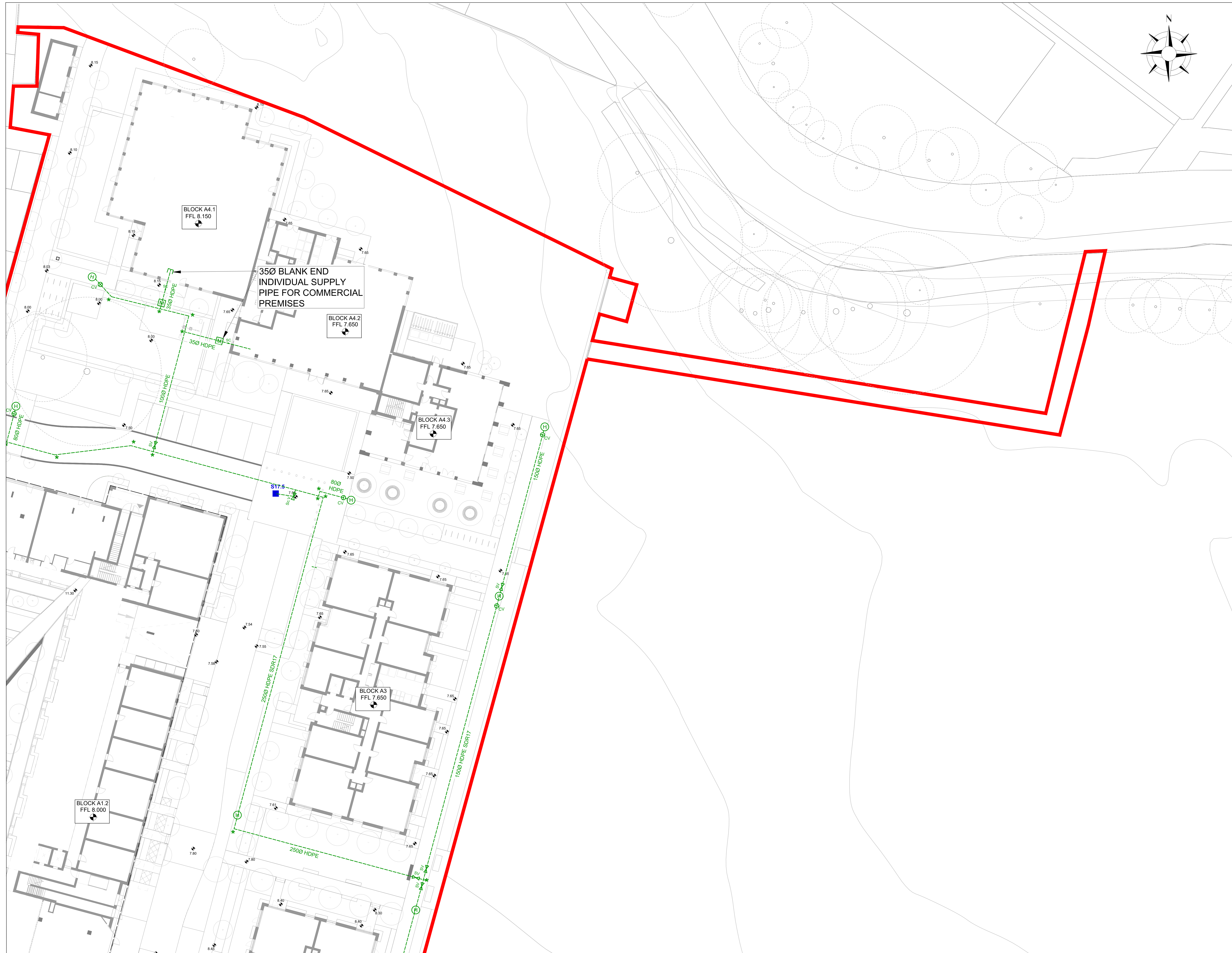
PROPOSED WATERMAIN SITE PLAN LAYOUT - SHEET 2 OF 8 SCALE @ A0: 1:200 SCALE @ A2: 1:400
